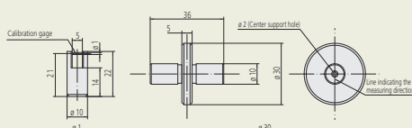
Calibration gage set for LSM-30-A
