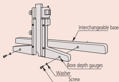
Mounting the interchangeable base
