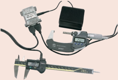
Sample application with footswitch (optional accessory)
