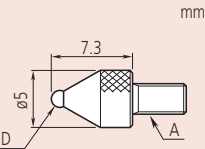
Ball point with attached ball
