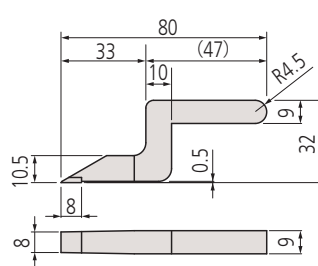
Scriber for height gages
