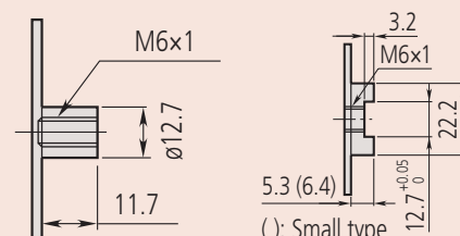
Unit : mm With screw mount
