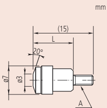
Flat point carbide (21AZB754)
