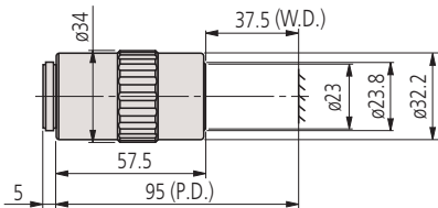
M Plan Apo NIR 5X
