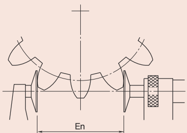
Root tangent length of gear (En)
