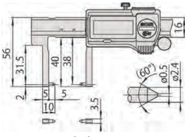
Point jaw type
