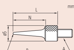
Needle Point
