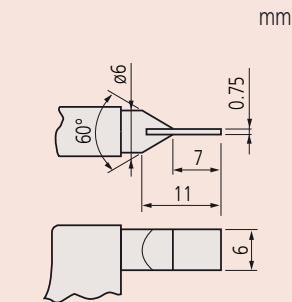
Type B (hardened steel)
