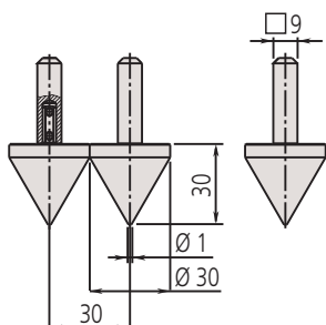
Centreline type
