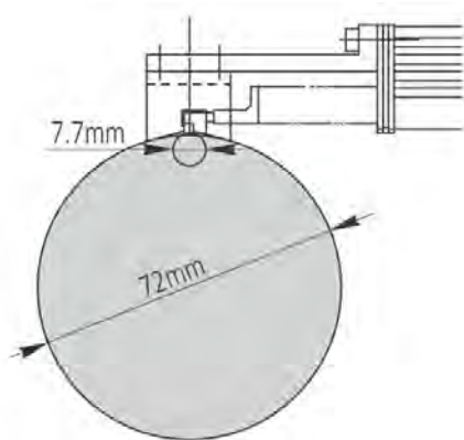
V-type adapter
