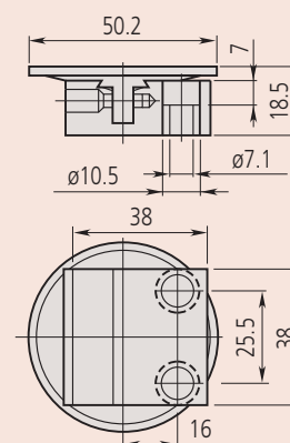
Unit : mm With adjustable bracket
