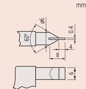
Type C (carbide-tipped)
