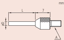
Cylinder Point
