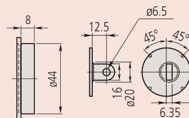
Unit : mm With magnet
