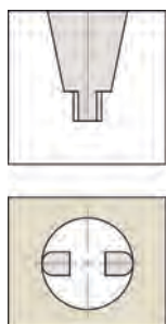
Round surfaces of jaws for measuring inside dimensions
