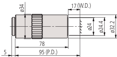
M Plan Apo NIR 50X
