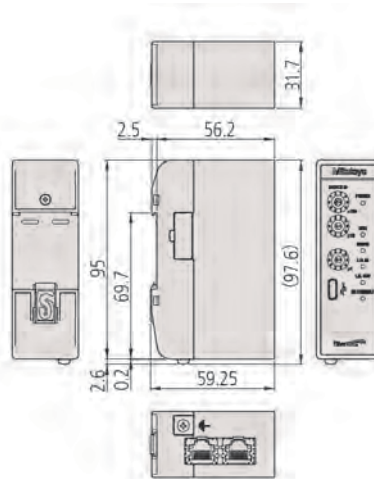
Interface unit EtherCAT (21HZA264)
