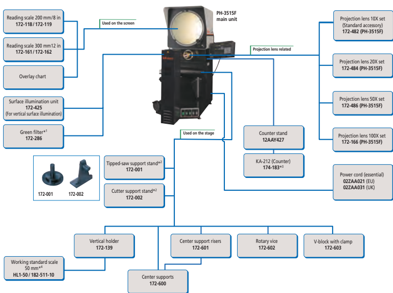
System Diagram
