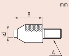
Flat point carbide (120056D)
