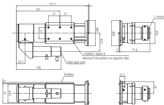
Dimensions VMU-T1
