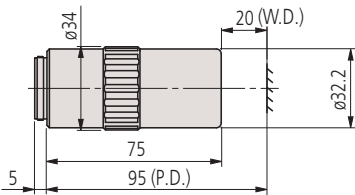
M Plan Apo NIR 20X
