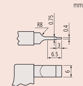
Type A (hardened steel)
