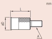
Flat point steel Flatness 3 μm
