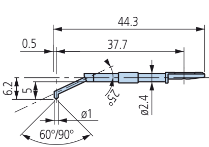
For hole bottom
