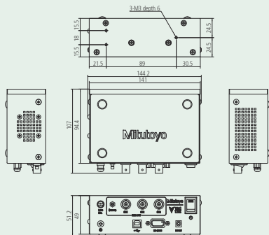
Controller Dimensions
