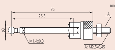
Lever Point
