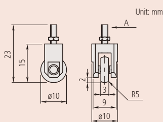
Roller point
