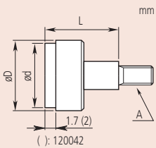
Flat point carbide (120041D)
