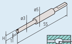
Small hole: 12AAM105 Tip shape: One-sided cut Tip angle: 20° Tip radius: 25 µm Tip material: Carbide
