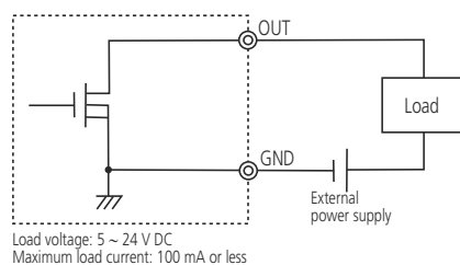
Circuit output
