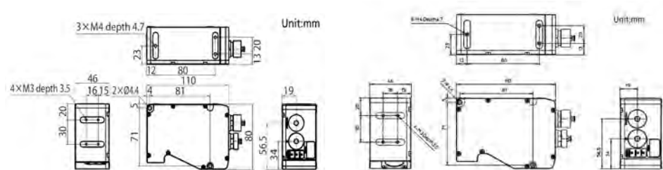
Mounting size SM1008S
