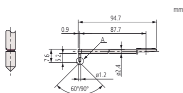
For deep hole [double-length]
