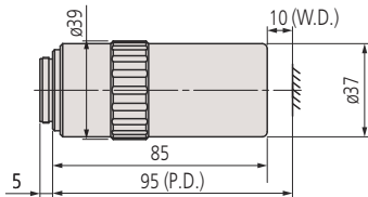
M Plan Apo NIR HR 100X
