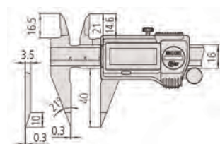
Fine measuring jaws
