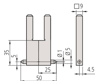
Inside point type
