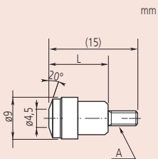
Flat point carbide (21AZB755)
