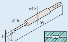
Small hole: 12AAM104 Tip shape: One-sided cut Tip angle: 20° Tip radius: 25 µm Tip material: Carbide
