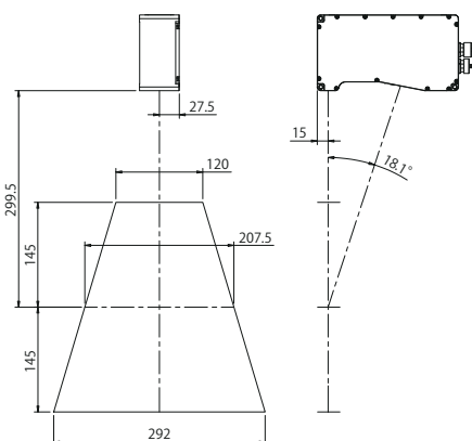
Measuring Range SM2929S (553-120)
