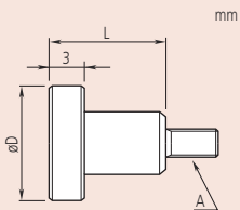
Flat point steel Flatness 5 μm
