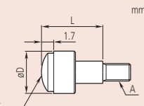
Spherical point carbide
