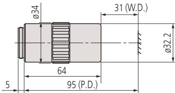
M Plan Apo NIR 10X
