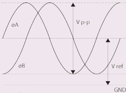
Output waveform
